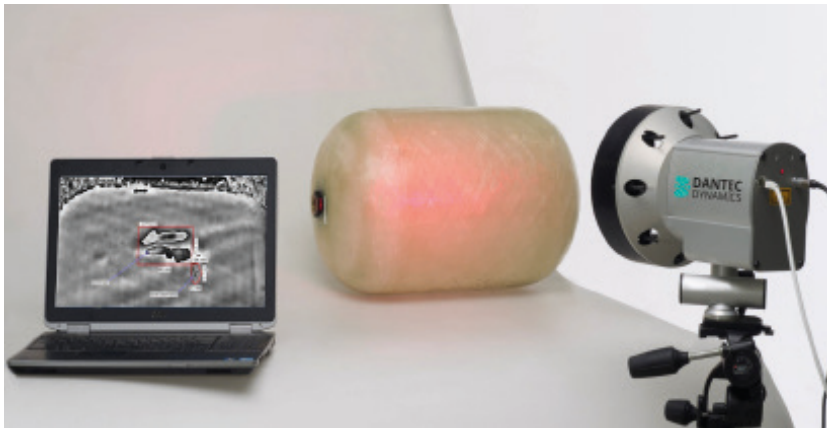
Shearography equipment
